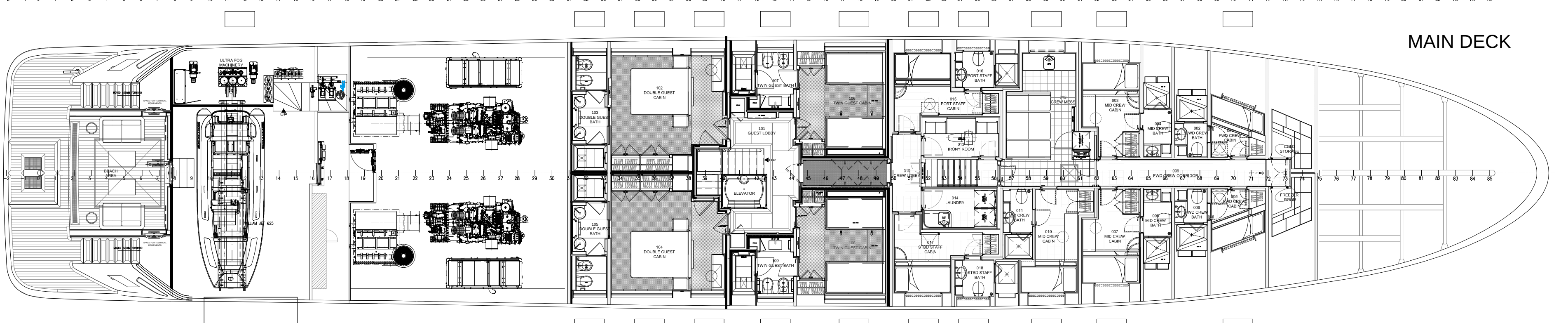
LOWER DECK
