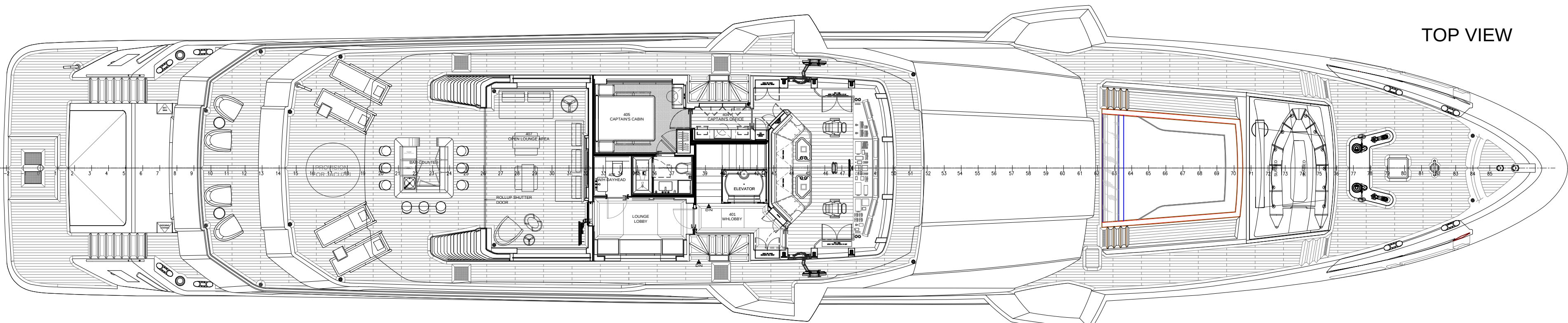
WHEELHOUSE DECK
